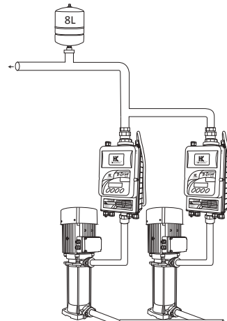
RDRIVE-PW Multibombeo
